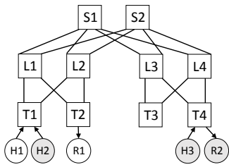
(a) Multi-bottleneck topology (b) Throughput of the three flows. F2 is the long flow (H2->R2)
