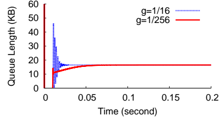
(a) 2:1 Incast
