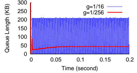
(b) 16:1 Incast
